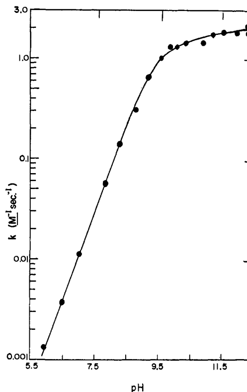
Figure 2. Plot of \log k_0 vs. pH for MEA with methyl iodide in water at 25°. [MEA] has been varied from 5.8 to 28.7 \times 10^{-4} M . The [\text{CH}_3\text{I}] has been varied from 5 to 18 \times 10^{-4} M . Much of these data are reported with all the experimental details and data in the thesis of S. P. Molnar.
