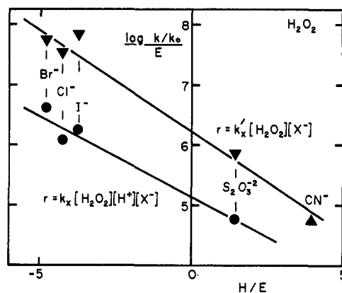
Figure 5. Oxibase scale plot of the reactions of various nucleophiles with hydrogen peroxide in water. The upper line is for the data in basic solution with a rate expression: \text{rate} = k'_x [\text{H}_2\text{O}_2][\text{X}^-] . The lower line represents the data obtained in an acidic medium where the rate expression is k_x [\text{H}_2\text{O}_2][\text{H}^+][\text{X}^-] .
