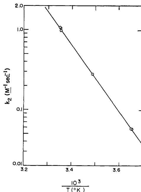
Figure 3. Temperature dependence of the reaction of \text{H}_3\text{N}^+\text{CH}_2\text{CH}_2\text{S}^- with methyl iodide in aqueous solution. \log k_2 vs. 1/T in a buffer of pH 9.90 \pm 0.02 .
